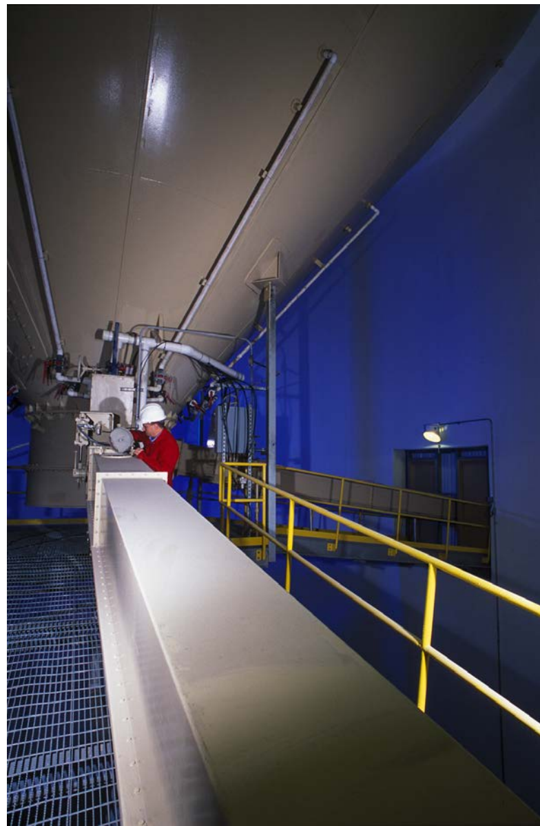
Airslide® gravity conveyor
